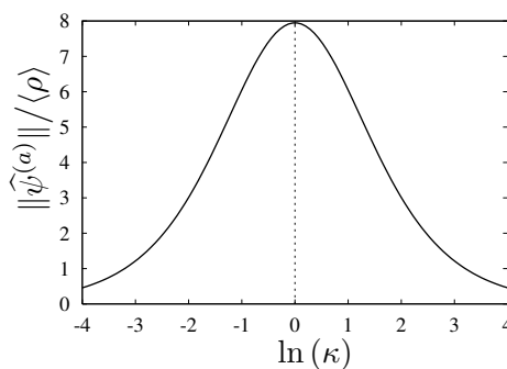
Figure 4: Colour zero modes \lambda_a
