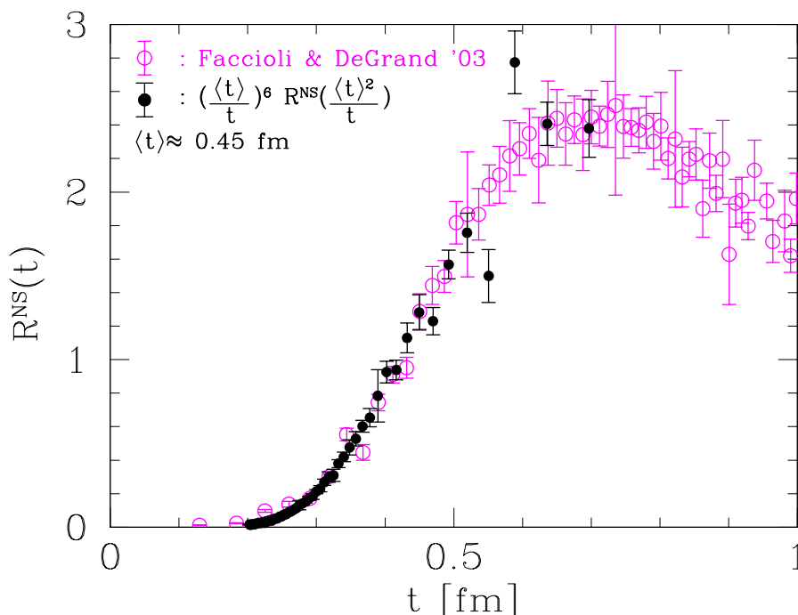
Figure 8: Alternative test of conformal (space-) time inversion symmetry for t \rightarrow \langle t \rangle^2/t , according to eqs. (4.1), (4.3) for the chirality-flip correlator R^{NS}(t) , using directly (quenched) lattice data from ref. [17]. The abscissa denotes Euclidean time in fermi. The agreement of the direct and overlaid data provides strong evidence that conformal (space-)time inversion holds also in the fermionic sector.
