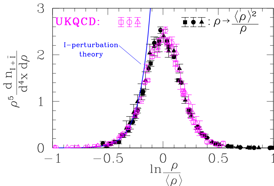
Figure 1: UKQCD lattice data [5, 6] (open symbols) for the instanton size distribution, displayed such as to suggest a virtually perfect inversion symmetry under \rho \rightarrow \langle \rho \rangle^2 / \rho with \langle \rho \rangle \approx 0.6 fm (open and solid data symbols fit onto one universal, symmetric curve). The solid line corresponds to the parameter-free prediction of instanton perturbation theory [6] using the lattice result \Lambda_{\overline{\text{MS}} n_f=0} = (238 \pm 19) MeV from the ALPHA collaboration [8].
