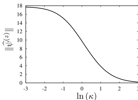
Figure 6: Translation zero modes
