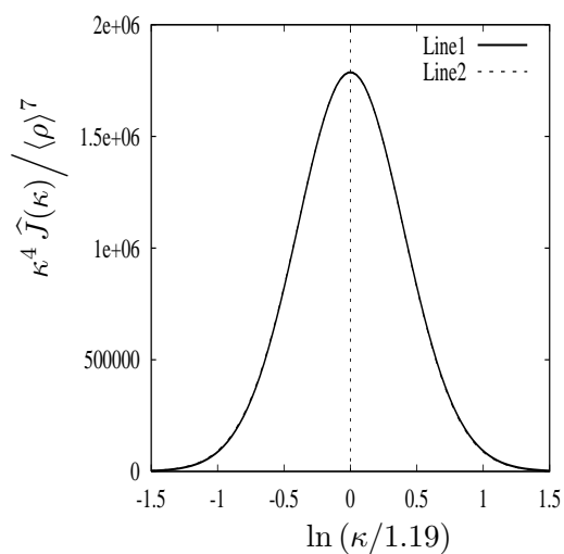
Figure 7: (Left): Total zero mode contribution \kappa^4 \widehat{J}(\kappa)/\langle\rho\rangle^7 times 1/\kappa on the sphere, as relevant for the instanton size distribution d(\rho\mu_\tau, \alpha_s) in eq. (2.11). As abscissa, we use \ln(\kappa/1.19) = \ln(\rho/(1.19\langle\rho\rangle)) to make small deviations from a perfect size inversion symmetry for \kappa/1.19 \leftrightarrow 1.19/\kappa self-evident. Line1 and Line2 display the results versus \kappa/1.19 and 1.19/\kappa , respectively. (Right): Same plot, but using a logarithmic ordinate, to demonstrate the high degree of inversion symmetry over fourteen orders of magnitude, with Line1 and Line2 being visually indistinguishable!
